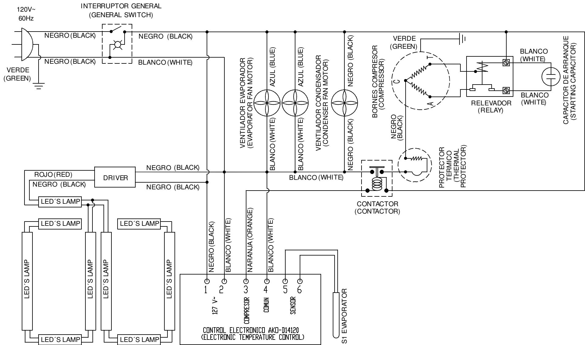
DIAGRAMA ELECTRICO (ELECTRIC DIAGRAM) RMH-40
